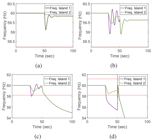
Figure B.1: Frequency disturbances during the black start due to unexpected increases in all the load buses by an adversary (as described in Section 4.2.2), ignoring generators' frequency cut-off limits (shown by red dashed lines). The maximum power outputs for the generators' governors are different in this figure from that of the generators in Fig. 11. (a) Normal black start operation in the absence of an adversary. (b) Demand increases of 10MW at the load buses before the reconnection of the two islands. (c) Demand increases of 20MW at the load buses before the reconnection of the two islands. (d) Demand increases of 30MW at the load buses before the reconnection of the two islands.
