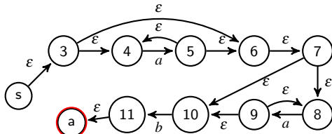
Figure 2: Automaton for the regular expression \text{/^a*a*b$/} . s is the starting state and a is the accepting state.
