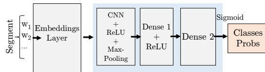
Fig. 4: Components of the CNN-based classifier used.
