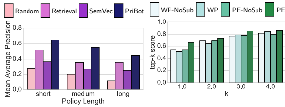
Fig. 10: top- k score of PriBot with different pre-trained embeddings.
