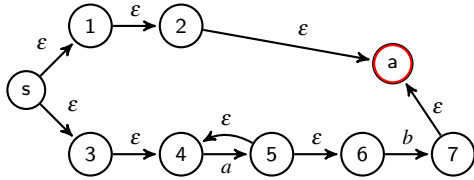
Figure 1: Automaton for the regular expression \text{/(a+b)?}/ . s is the starting state and a is the accepting state.
